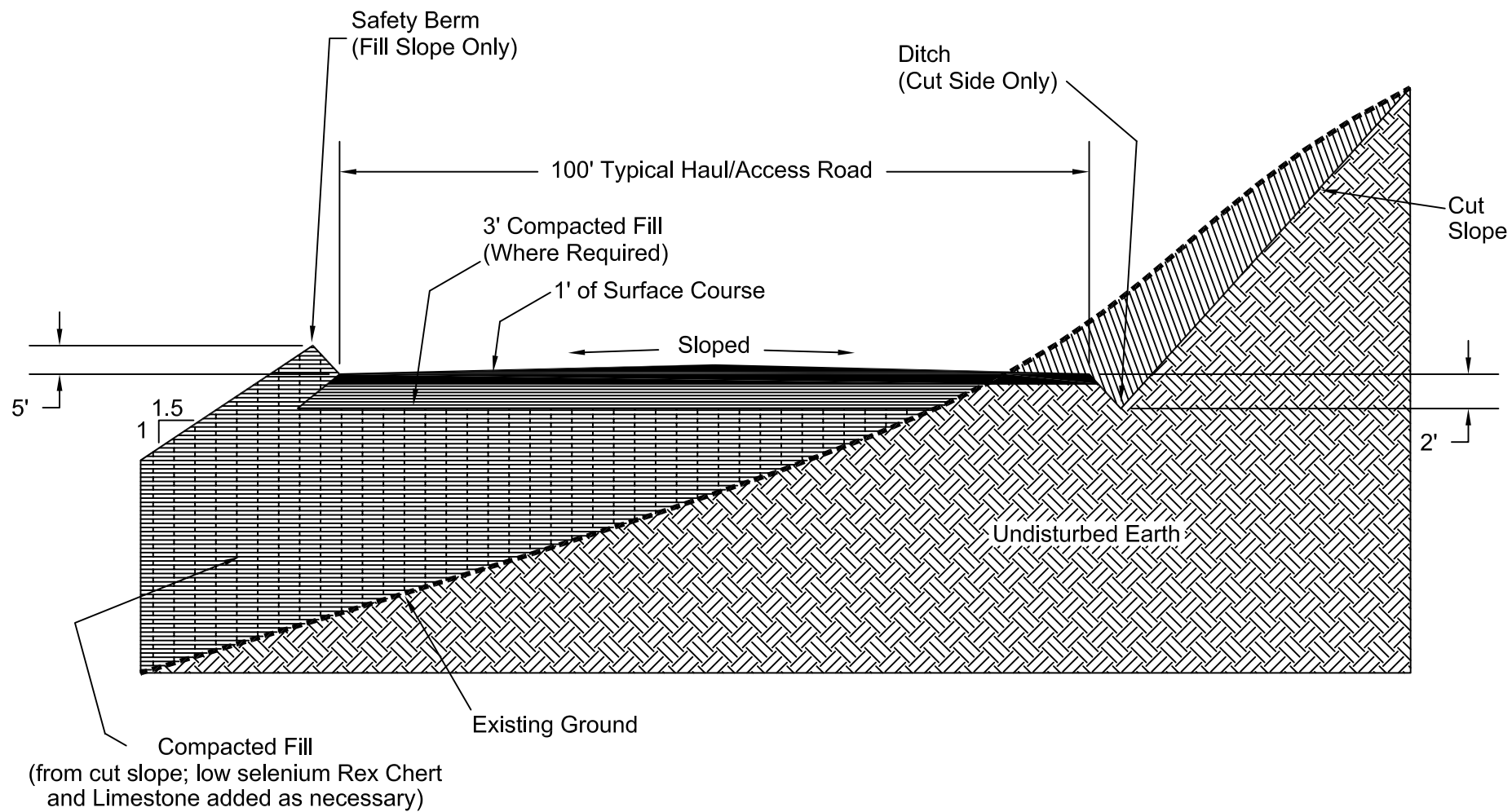
Figure 2.4-2 Typical Haul/Access Road Smoky Canyon Mine Panels F and G
