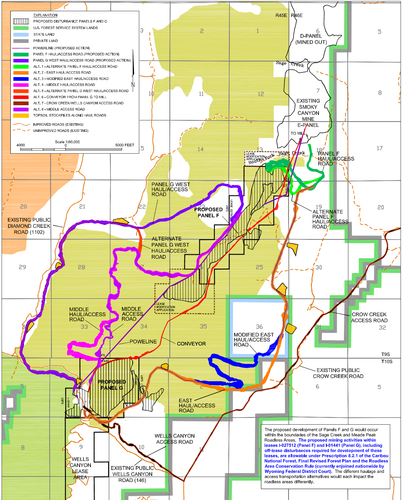
Figure 2.6-9 Transportation Alternatives with IRAs Smoky Canyon Mine Panels F and G
